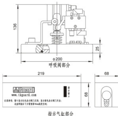
Fitting Details
