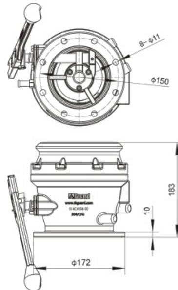
Fitting Details
