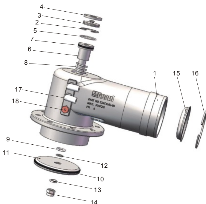
Part Drawing
