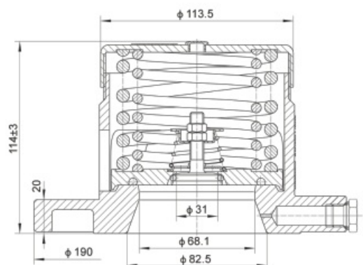
Fitting Details
