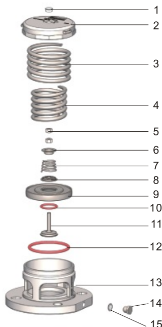
Part Drawing
