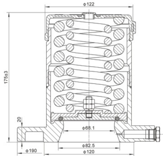
Fitting Details
