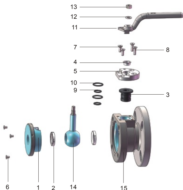
Part Drawing
