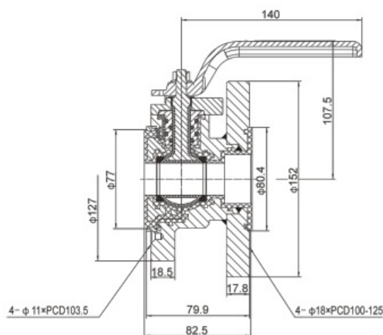
Fitting Details
