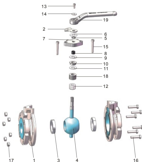
Part Drawing
