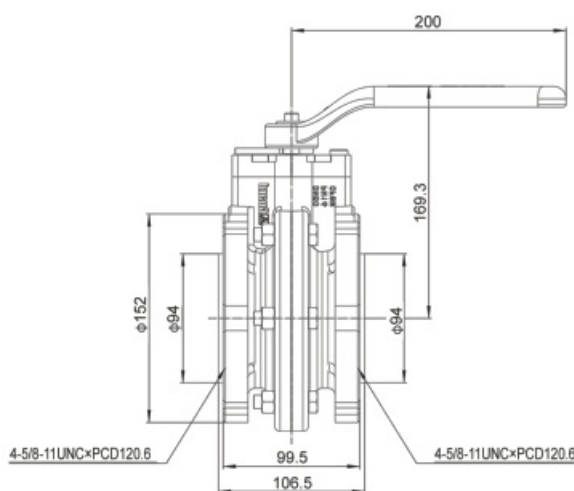
Fitting Details
