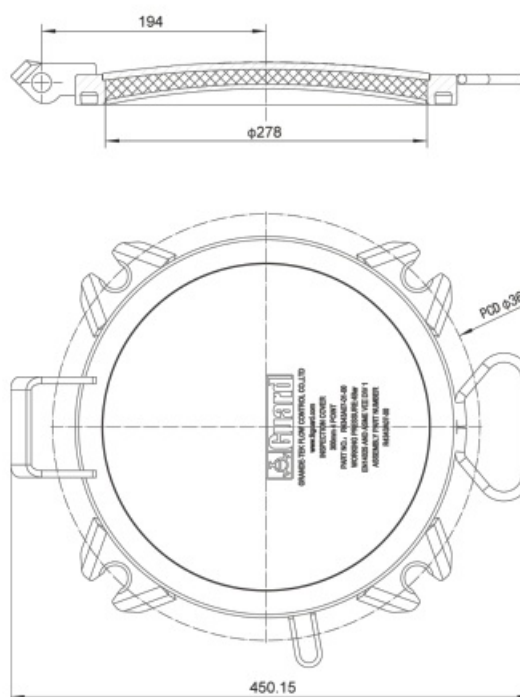
Fitting Details
