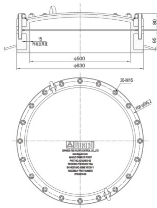
Fitting Details
