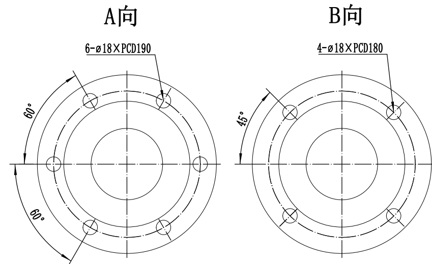
Connection Flange
